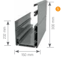
Gutter (Water-drain)
