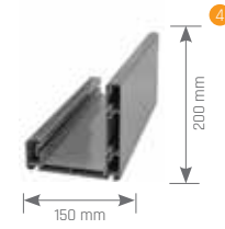
Gutter (Water-drain)
