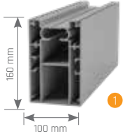
Rails
